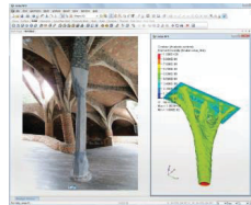
Shape Optimisation Bridge Pier
