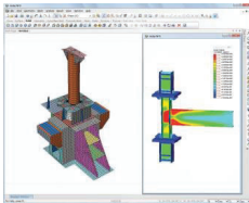
Static/Fatigue Analysis Steel structure's connection
